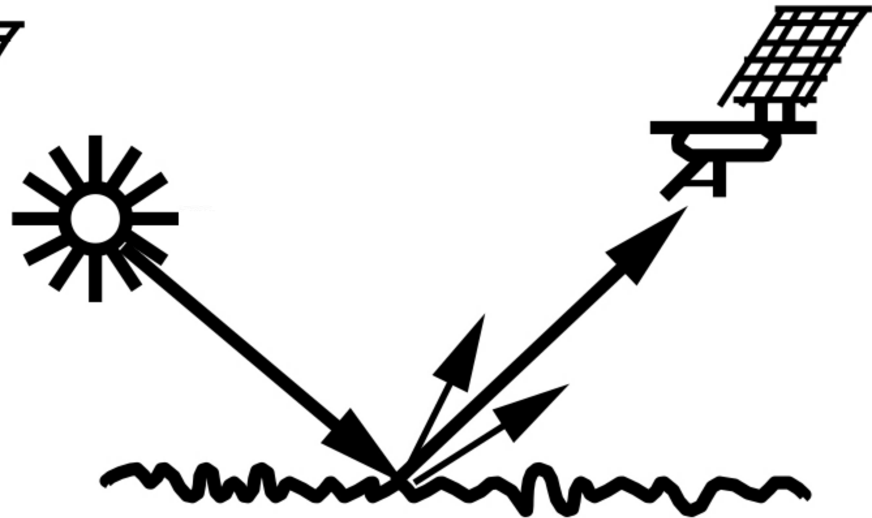
Rough water surface BRDF: sun glint reflectance
