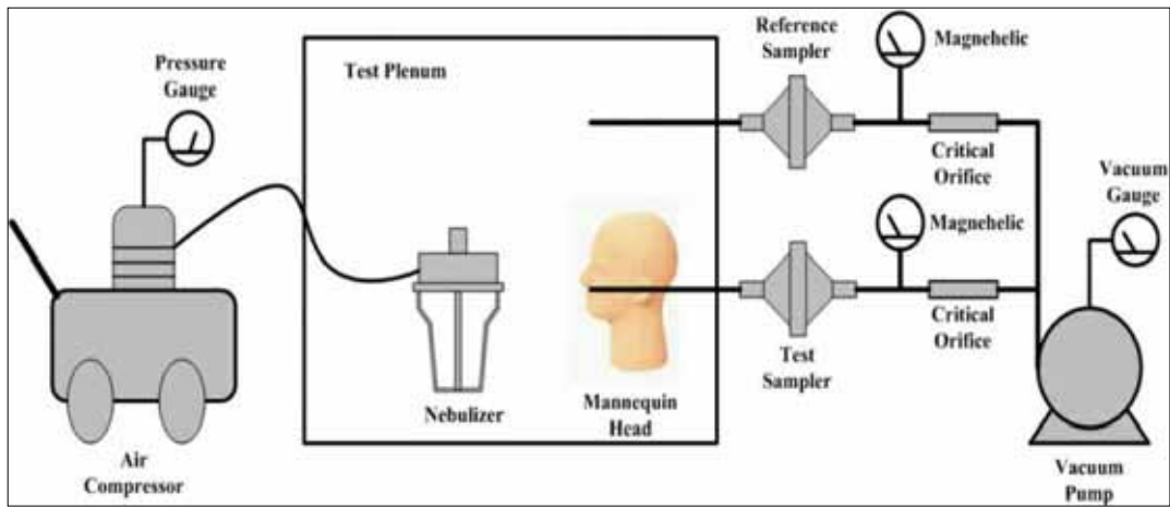
Figure 1 Face Mask Test System
